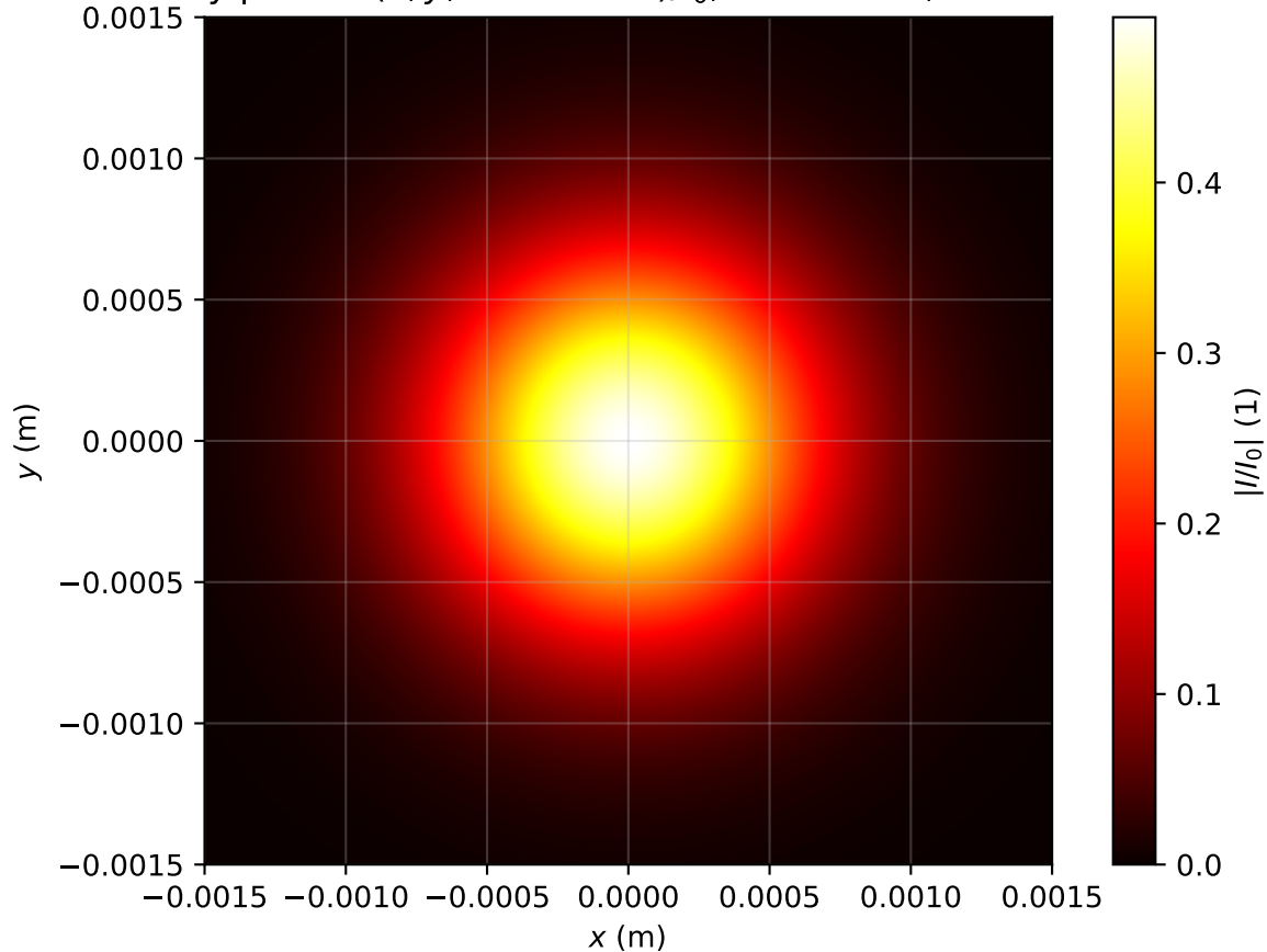
Intensity profile I(x, y, z = 2.627m)/I_0 , Pin=0.3Pcr, artificial time
